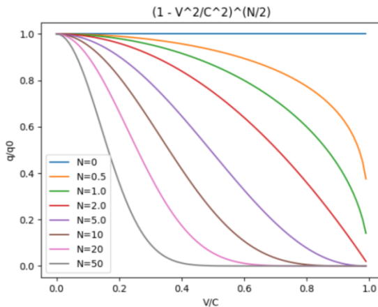
Fig.2 : q / q_0 is a function of v / c for a numbers of values of N : 0 , 0.5 , 1.0 , 2.0 .... In the external field represented by N , the effective electric charge of the electron decreases toward zero as v tends to c .
