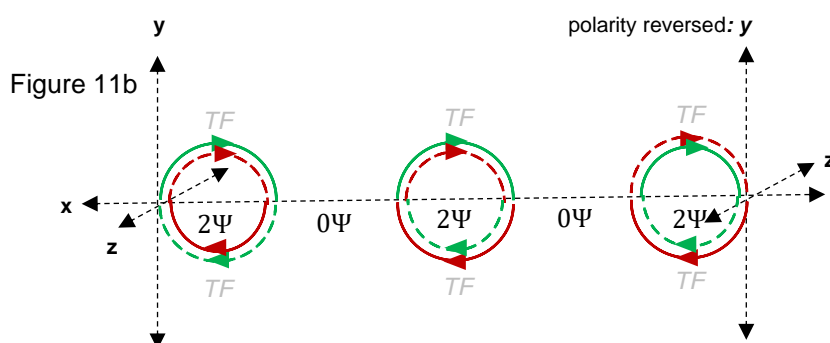
Figures 11a-11b: temporal “phase-3” as the green and red quasiparticles forming from their basic time-forward (TF) and time-reverse (TR) wave function ( \Psi ) components (11a) to their time-forward (TF) adjusted wave function ( \Psi ) components (11b).
