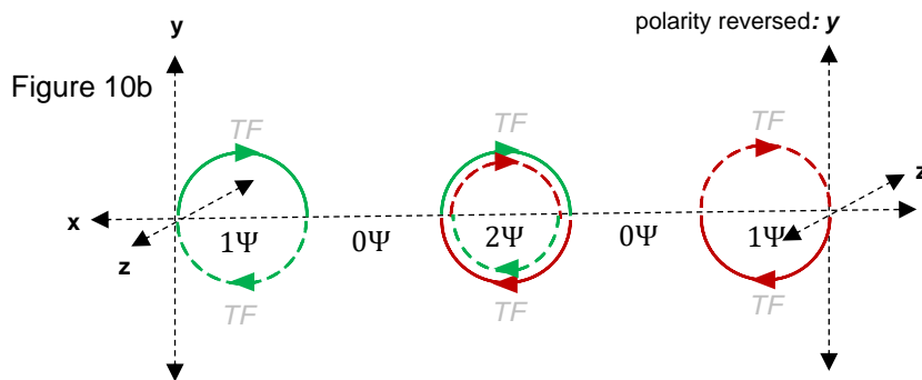
Figures 10a-10b: temporal “phase-2” as the green and red quasiparticles forming from their basic time-forward (TF) and time-reverse (TR) wave function ( \Psi ) components (10a) to their time-forward (TF) adjusted wave function ( \Psi ) components (10b).
