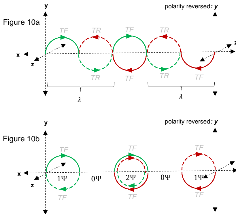
Figures 10a-10b: temporal “phase-2” as the green and red quasiparticles forming from their basic time-forward (TF) and time-reverse (TR) wave function ( \Psi ) components (10a) to their time-forward (TF) adjusted wave function ( \Psi ) components (10b).
