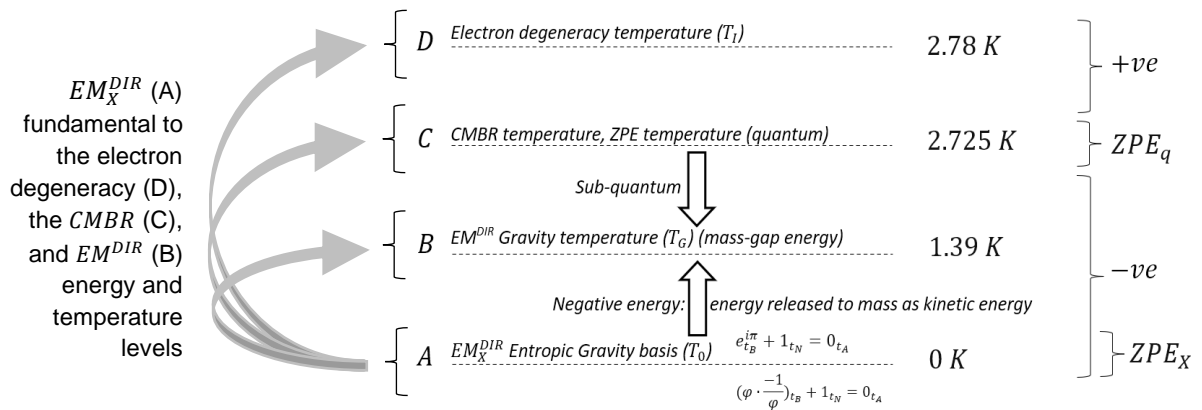
Figure 17: note here how EM_X^{DIR} level A is fundamental to the electron degeneracy level D, the CMBR level C, and EM^{DIR} level B, and thus would in theory have certain energy requirements for its manifestation to instruct the behaviour of levels B→D
