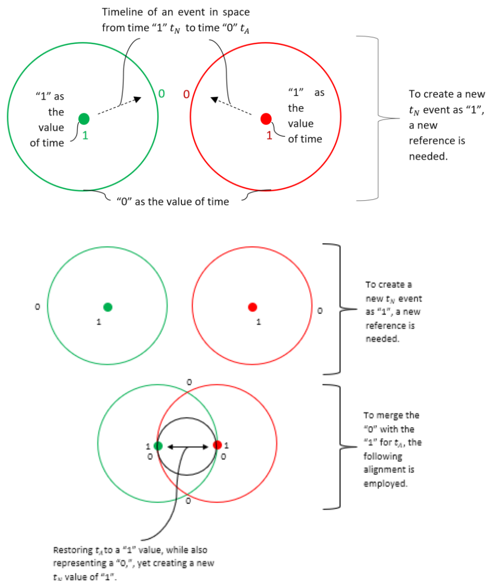
Figure 3: a basic schematic description for the Majorana particle/field, as the amalgamation of the properties of \varphi and -\frac{1}{\varphi}
