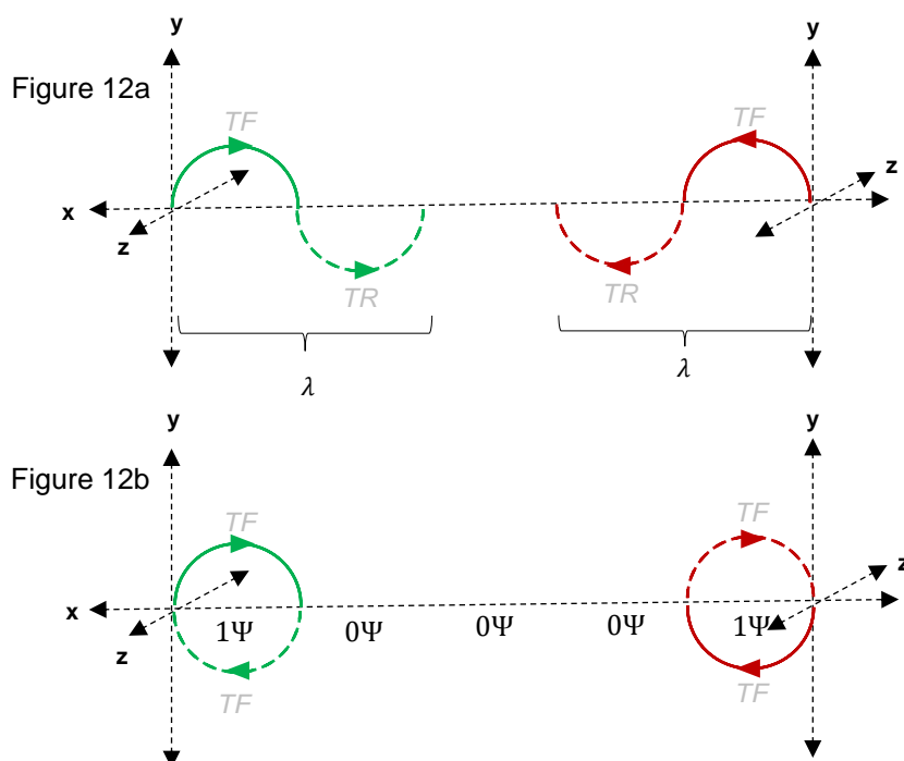
Figures 12a-12b: temporal "phase-1" as the green and red quasiparticles forming from their basic time-forward (TF) and time-reverse (TR) wave function ( \Psi ) components (12a) to their time-forward (TF) adjusted wave function ( \Psi ) components (12b).
