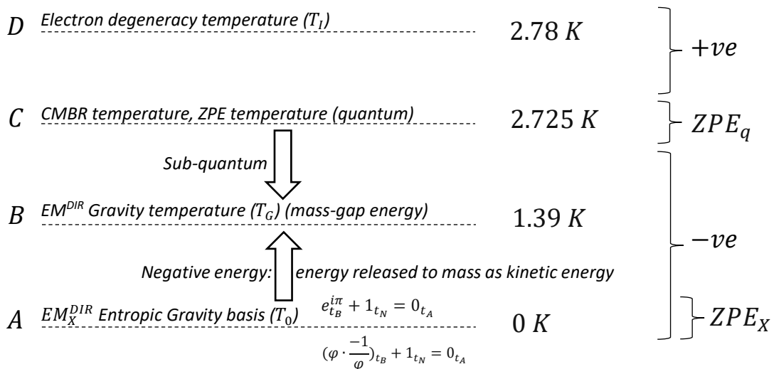
Figure 1: EM_X^{DIR}/ZPE_X entropic gravity basis as T_0 (A), EM^{DIR} gravity temperature T_G (B), CMBR/ ZPE_q temperature (C), electron degeneracy temperature T_I (D).
