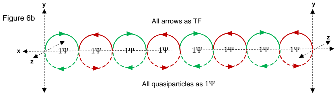
Figures 6a-6b: temporal “phase-2” as the green and red quasiparticles forming from their basic time-forward (TF) and time-reverse (TR) wave function ( \Psi ) components (6a) to their time-forward (TF) adjusted wave function ( \Psi ) components (6b).
