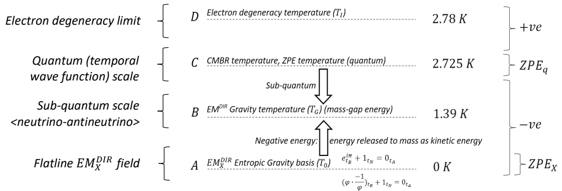
Figure 2: flatline EM_X^{DIR} field (A), the sub-quantum EM^{DIR} scale as the neutrino/antineutrino level (B), the EM quantum temporal wave function scale (C), the electron degeneracy temperature limit (D).
