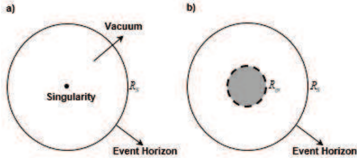
Figure 3: a) Existing Model. b) New Model. The area of within R_{gs} (or R_{gs-vir} ) has gravitational self-energy (potential energy) of negative value, which is larger than mass energy of positive value. If r is less than R_{gs} , this area becomes negative energy (mass) state. There is a repulsive gravitational effect between the negative masses, which causes it to expand again. This area (within R_{gs} ) exercises anti-gravity on all particles entering this area, and accordingly prevents all masses from gathering to r=0 . Therefore the distribution of mass (energy) can’t be reduced to at least radius R_{gs} (or R_{gs-vir} ).
