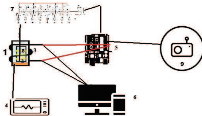
Fig.10: HMC with DAC and feedback
