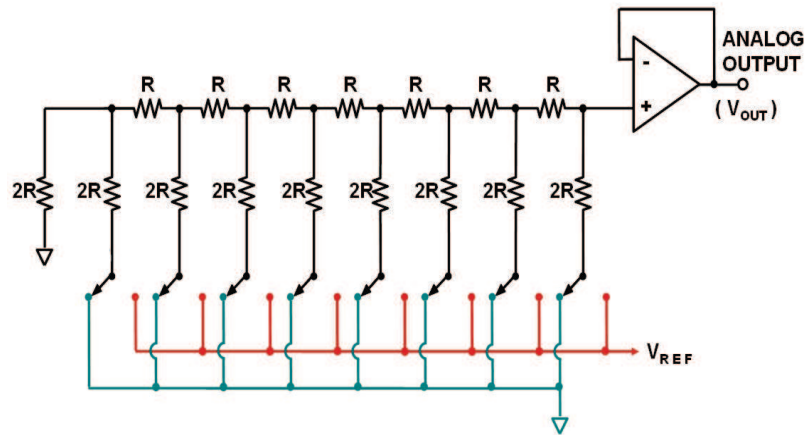
Fig.8: DAC scheme
