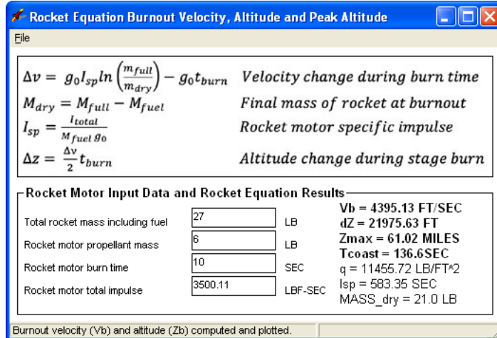
Figure-8, Burnout velocity (Vb), burnout altitude (Zb), peak altitude (Zmax) and coast time to peak altitude (Tcoast) for a hypothetical rocket is computed using the rocket equation .
