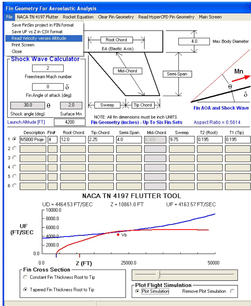
Figure-9, Enhanced Fin Geometry screen available in FinSim 10 or greater for the Supersonic Rocket fin flutter example. The rocket's burnout velocity is the red dot with the Vb designation on the UF versus Z (altitude) plot.
