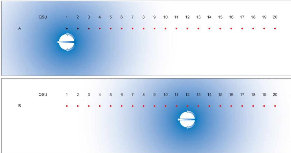
Figure 5- Reference frame and \psi motion diagram. The white dot at the center of the figure represents the reference frame, and the blue surrounding the white dot represents \psi . The blue arrows indicate the \psi contracting around the body, moving the body forward.
