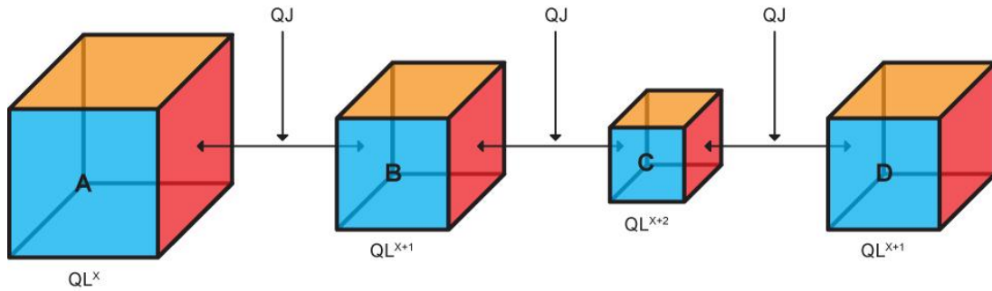
Figure 5- QL State Function of the D-string. A D-string undergoes three quantum jumps with an initial arbitrary value of x , denoted as QL^x , as in cube A. The D-string quantum jumps and contracts from QL^x to QL^{x+1} as in cube B. The D-string now undergoes a quantum jump and contracts a second time to QL^{x+2} as in cube C. Finally, the D-string Quantum jumps and expands to QL^{x+1} as in cube D. Though the D-string has undergone three quantum level changes, the net change in the D-string quantum level is one QL . It is not the number of Quantum jumps a D-string undergoes that determines quantum level, but it is the net difference in quantum jumps from the initial to the final quantum level.
