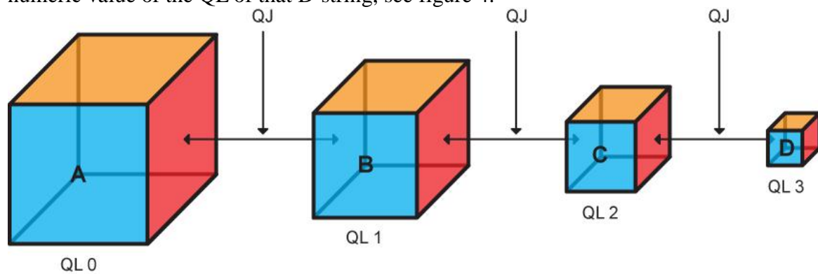
Figure 4- Quantum level changes with successive quantum jumps: Cube A represents a D-string in the fully expanded state, and cubes B, C, and D in progressive QJ contracted geometric configurations illustrate the QL of a D-string at each subsequent QJ. The final QL is the net total number of QJs from the maximally expanded state of the D-string. The sizes of the QL contractions in figure 4 are greatly exaggerated for clarity.
