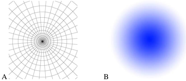
Figure 4 - (A) The 2-dimensional figure represents a space-time field of concentric QLs of a body (QL size exaggerated for clarity). (B) The 3-dimensional graphic represents a space-time field differential surrounding a body.
