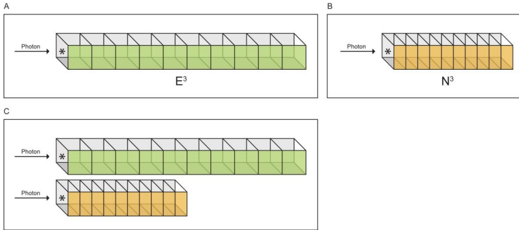
Figure 7- Euclidean ( E^3 ) and Non-Euclidean ( N^3 ) Geometries; (A) Euclidean reference frame with fully expanded D-strings having equal lengths along x, y, and z-axes with the time required to traverse 10 fully expanded D-strings equaling 10 \times T_p = 10 T_p , and the distance traversed equaling 10 \times L_p = 10 L_p . (B) Non-Euclidean reference frame with warped or contracted space-time with D-string axes not equal in length. The D-strings in this case are contracted \frac{1}{2} in direction of motion. The time to traverse ten contracted D-strings equals, 10 \times T_p = 10 T_p and the distance traversed equals, 10 \times \frac{1}{2} L_p = 5 L_p . (C) E^3 juxtaposed to N^3 - the photon will appear to move at half the speed and move half the distance in N^3 as compared to E^3 .
