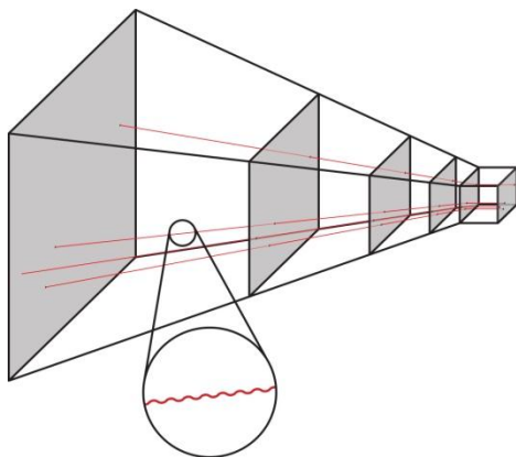
Figure 6- Space-time warpage by Particle Matter- The cube represents a quantum particle of matter. The non-cubic hexahedrons represent the D-strings s of space-time. The strings of the D-strings abutting the quantum particle warp the D-strings when aligning with strings of the particle matter. The strings of the strings warp the strings?
