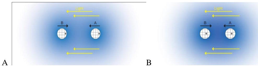
Figure 8- (A) shows two bodies A and B moving in opposite directions and at the same speed, as indicated by the black bars above the bodies. Photons from a light source coming from the same direction as body A enter the reference frame of body A and body B at the same instant, as indicated by the asterisk. Figure (B) shows that since both bodies are moving at the same speed, the bodies have identical space-time densities of their respective reference frames, and the photons of both bodies propagate at the same rate of one D-string per Planck's time. An observer within the reference frame of either body A or B will observe the speed of light at the same speed, despite moving in opposite directions from the light source.
