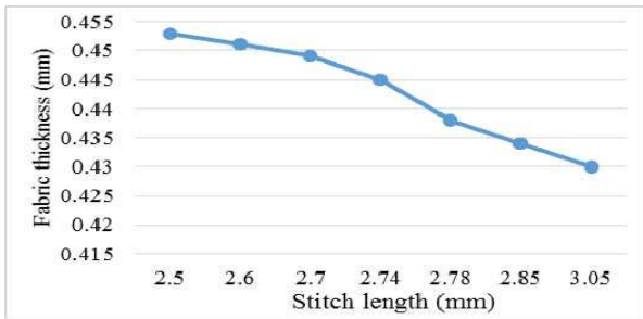
Figure 2: Change of Fabric Thickness with stitch length
