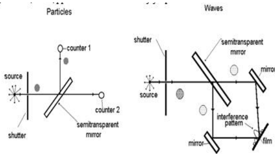
Figure 1 Experiments with individual photons on semitransparent mirror.
