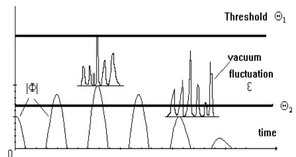
Figure 4 Quantum measurements
