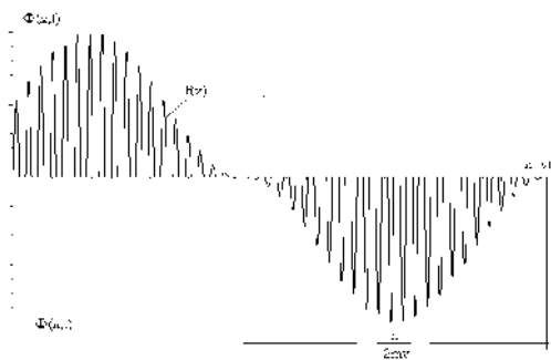
Figure 2 Behavior of wave packet in linear dispersion medium (i.e., rather like a series of stroboscopic photographs).
