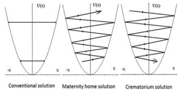
Figure 6 Decisions for harmonic oscillator in UKT
