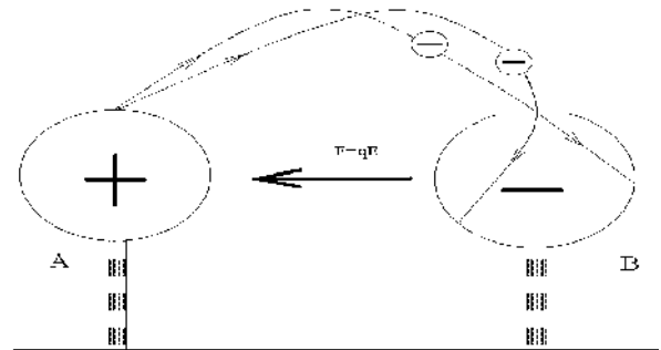
Figure 7 Work for transferring the charge depends on the mode of transferring and on the path.
