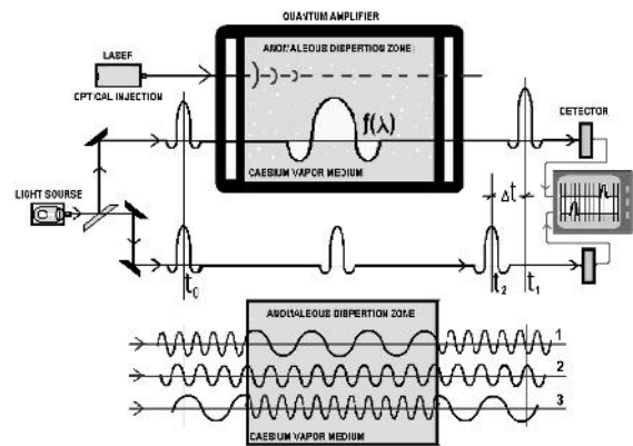
Figure 5 Experiments of L.Wang - superluminal light propagation
