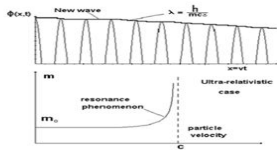
Figure 3 Dependency of the mass of the particle from velocity
