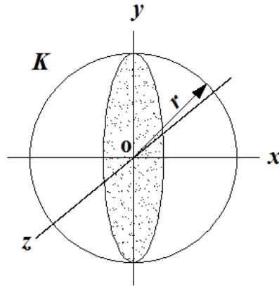
Fig.1. After a time t > 0 a sphere of light of radius r = ct expands in inertial system K . All positions on the x -axis within the sphere record the same time t and the same radius r = ct . The expanding great circle of light in the y - z plane (shaded area) has the same radius as the wavefront on the x -axis.
