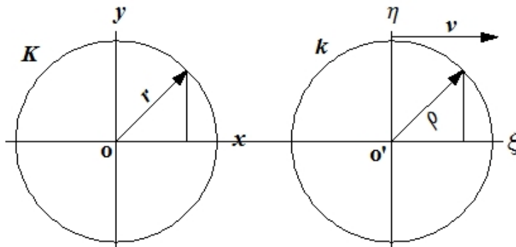
Fig.3. Einstein’s scenario: after a time t > 0 the expanding spherical wave of light has radius r = ct in system K and \rho = c\tau in system k . At t = \tau = 0 the two systems are superposed (so their origins coincide) when the light wave is emitted in all directions. The origins are separated by the distance d = vt according to system K .
