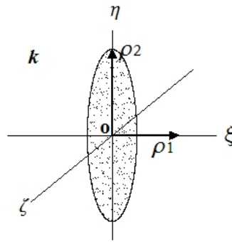
Fig.4. The radius \rho_2 = c\tau of the expanding light-circle in the \eta - \xi plane (shaded area) is not the same as \rho_1 = c\tau of the light wavefront on the \xi -axis in the direction of motion v , because the respective times \tau are not the same since time depends upon position \xi in system k under Lorentz Transformation from system K .
