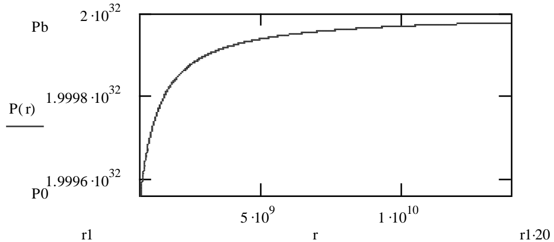
Fig.2. Radial distribution of ether pressure for the Sun.
