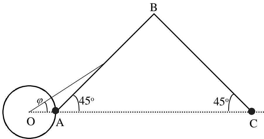
Figure 3. Schema of the flight to the moon, where O – Earth and C – Moon
