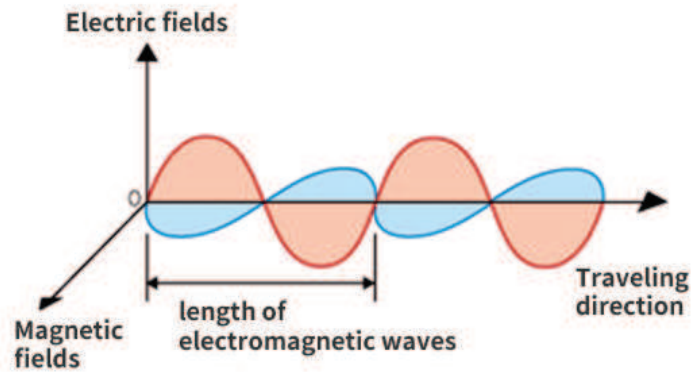
Electromagnetic wave (including visible light)
