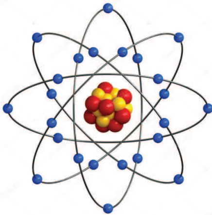
Rutherford planetary model
