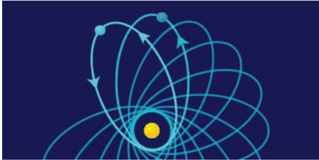
The precession of Mercury orbit.
