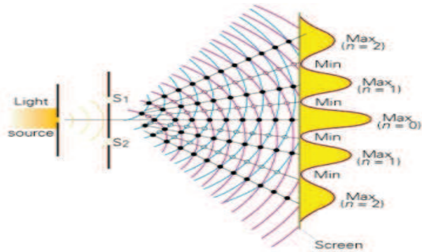
Double slit experiment
