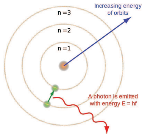
Bohr electron's photon emission
