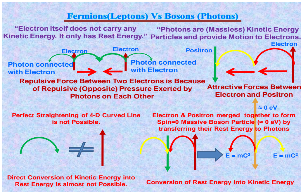
Fig. 10: Horizontal Massless Bosons i.e. Photons (Kinetic Energy) of Massive Charged Fermions (Rest Energy)
