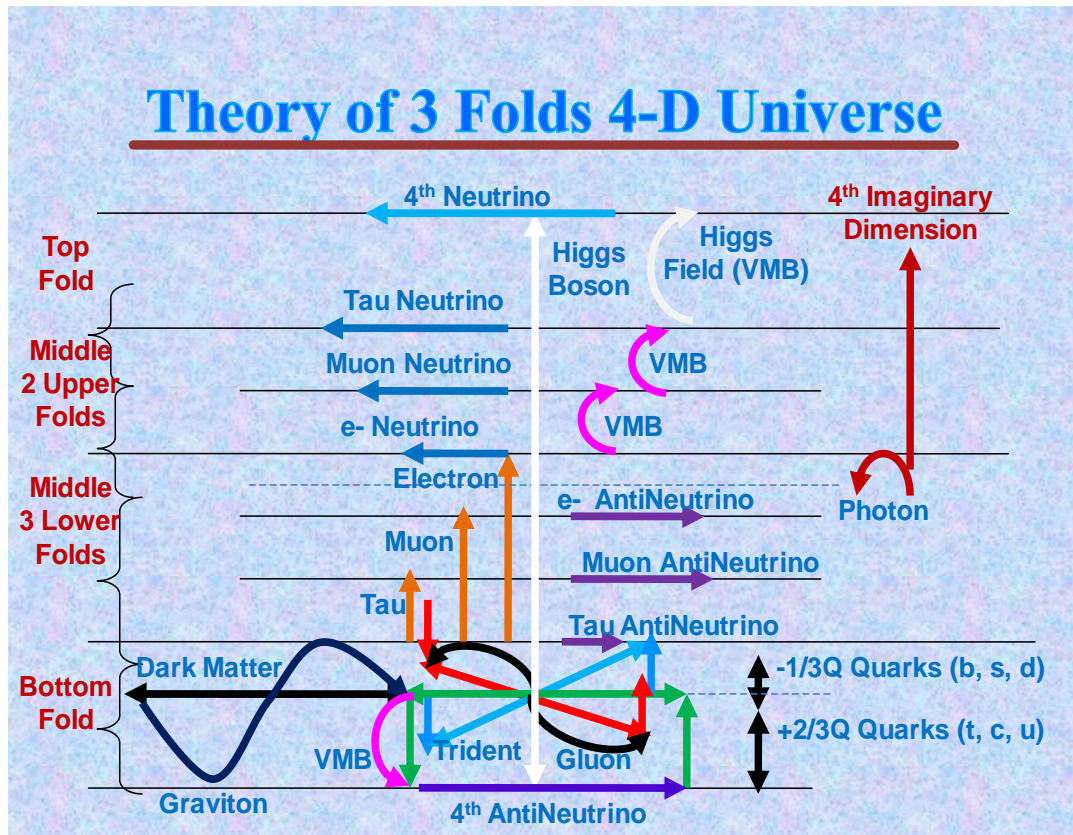
Fig. 16: Arrangement of All Fundamental Particles in their Respective Folds
