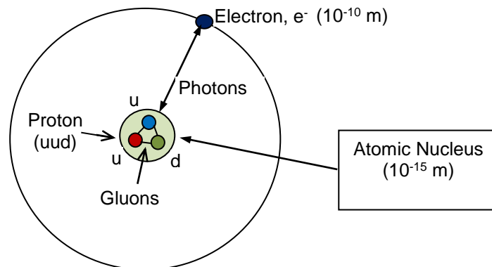
Fig. 1: Hydrogen Atom
