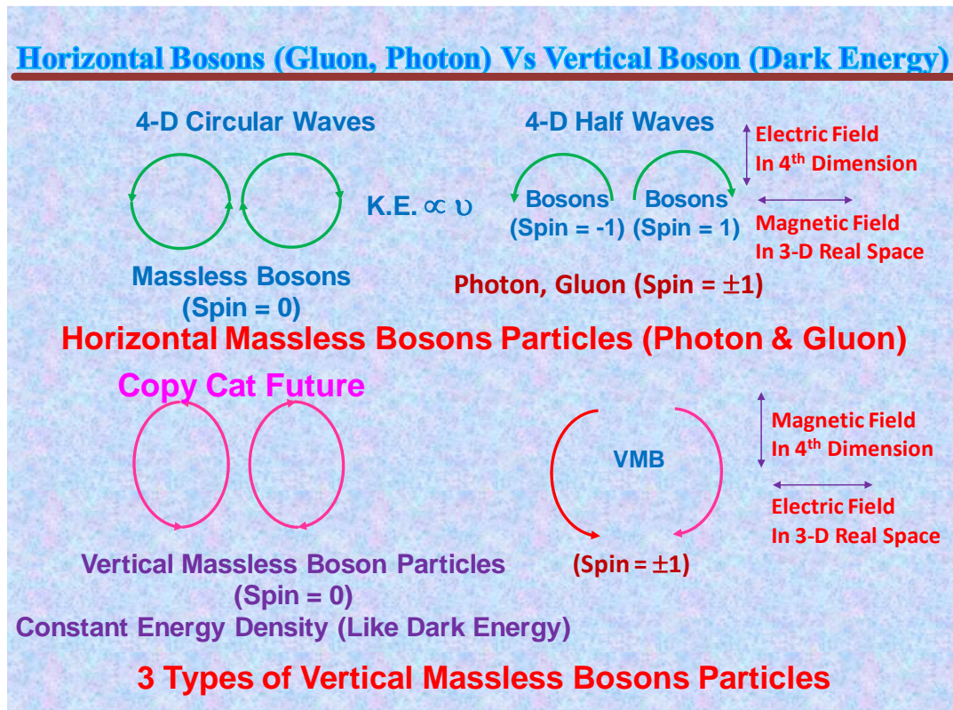
Fig. 11: Horizontal Massless Bosons Particles Vs Vertical Massless Bosons Particles
