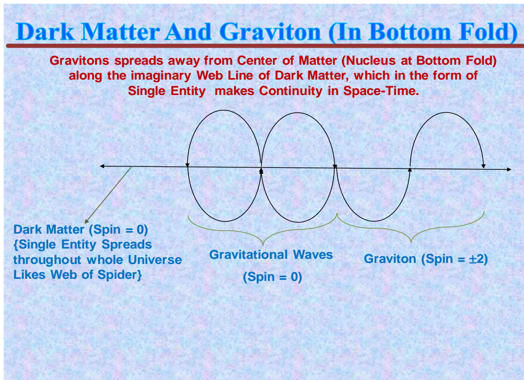
Fig. 8: Dark Matter (Single Entity Like Web of Spider) And Gravitational Waves (Spin= 0)
