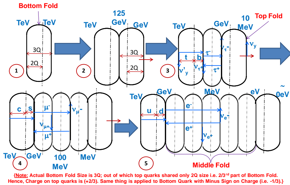
Fig. 5: Creation of 3 Folds and Fundamental Particles in 4 th Imaginary Dimension
