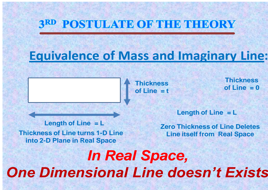
Fig. 2: Nature of One Dimensional Line in Real Space
