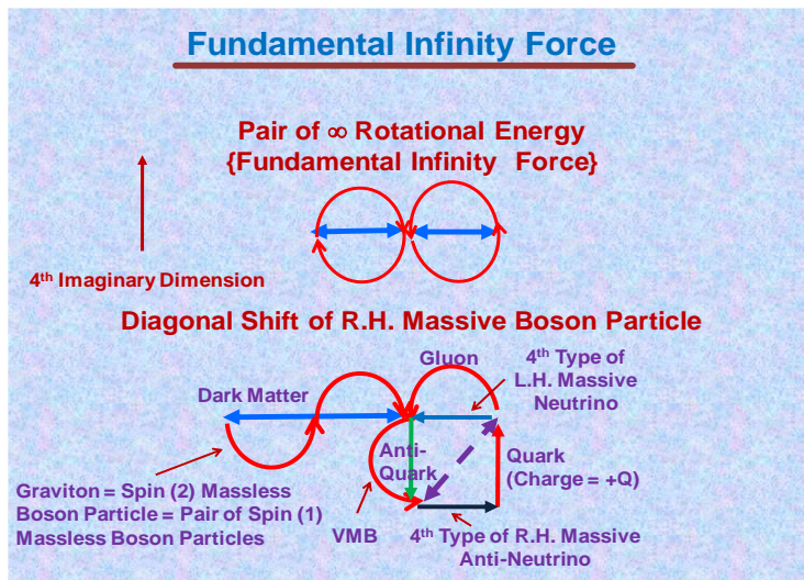
Fig. 14: Infinity (∞) Like Rotation of Massless Boson (Spin=0) Particles at TeV Range
