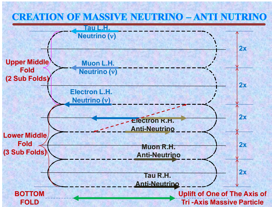
Fig. 12: Creation of Pair of Massive Neutrinos and Antineutrinos
