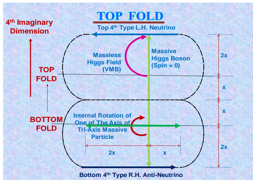
Fig. 13: Creation of Top Fold
