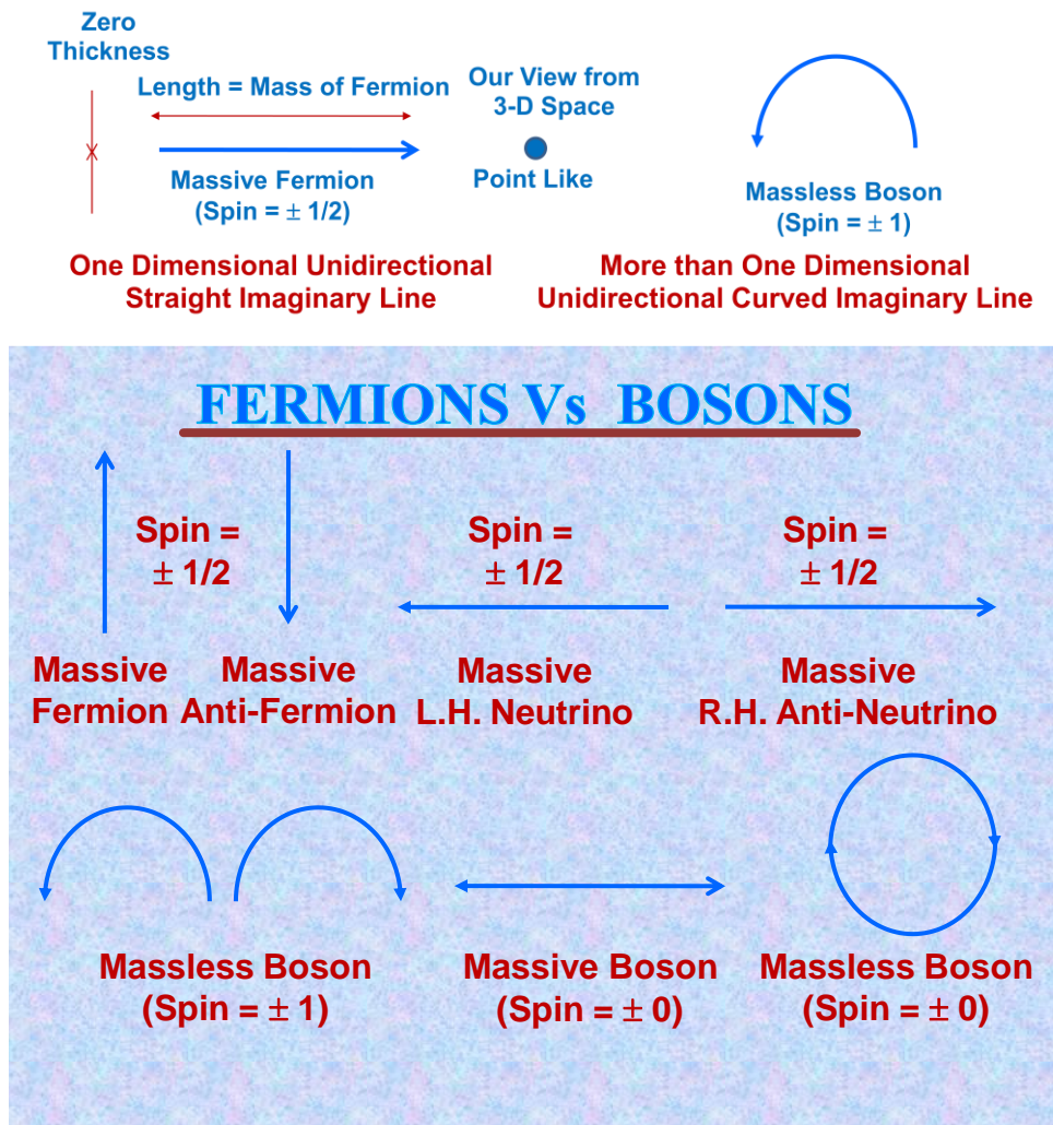
Fig. 3: Massive Fermions Vs Massless Bosons
