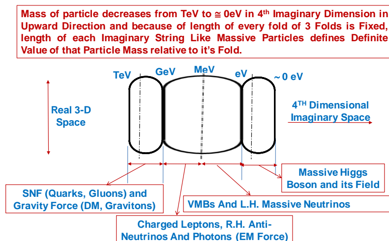
Fig.4: Arrangement of Fundamental Particles (3 Folded Way) in 4 th Imaginary Dimension
