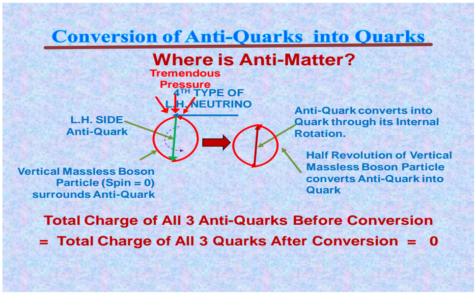
Fig. 7: Conversion of Anti-Quarks (Anti-Matter) into Quarks (Matter)
