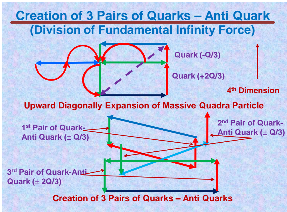
Fig. 15: Creation of 3 Pairs of Quarks-Anti Quarks and Trident Particle in Bottom Fold
