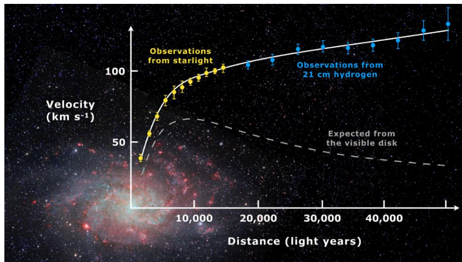
Figure 33. 'Flat' Galaxy Rotation Curves Interpreted as 'Dark Matter' 17
