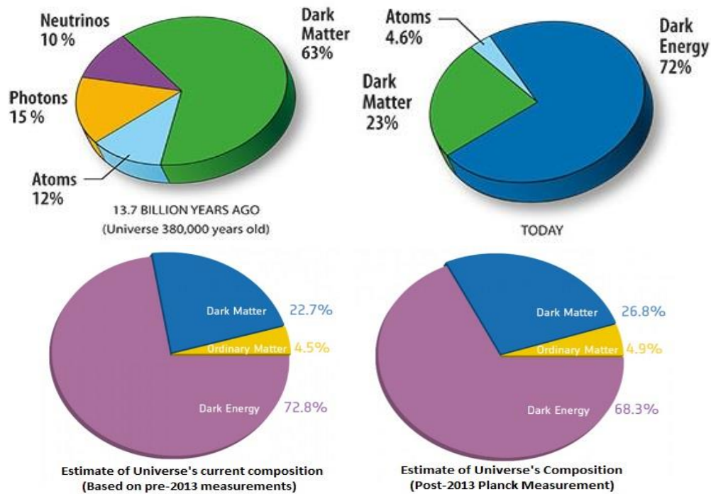
Figure 4. Changes in Universe's Hypothesized Composition given Observations [44, 121]
