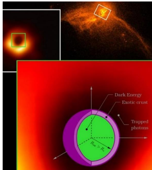
Figure 57. Croker & Weiner's Black Hole Dark Energy Hypothesis 32
