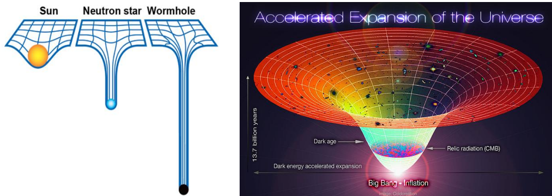
Figure 56. The Big Bang as a Gravity Well 31
