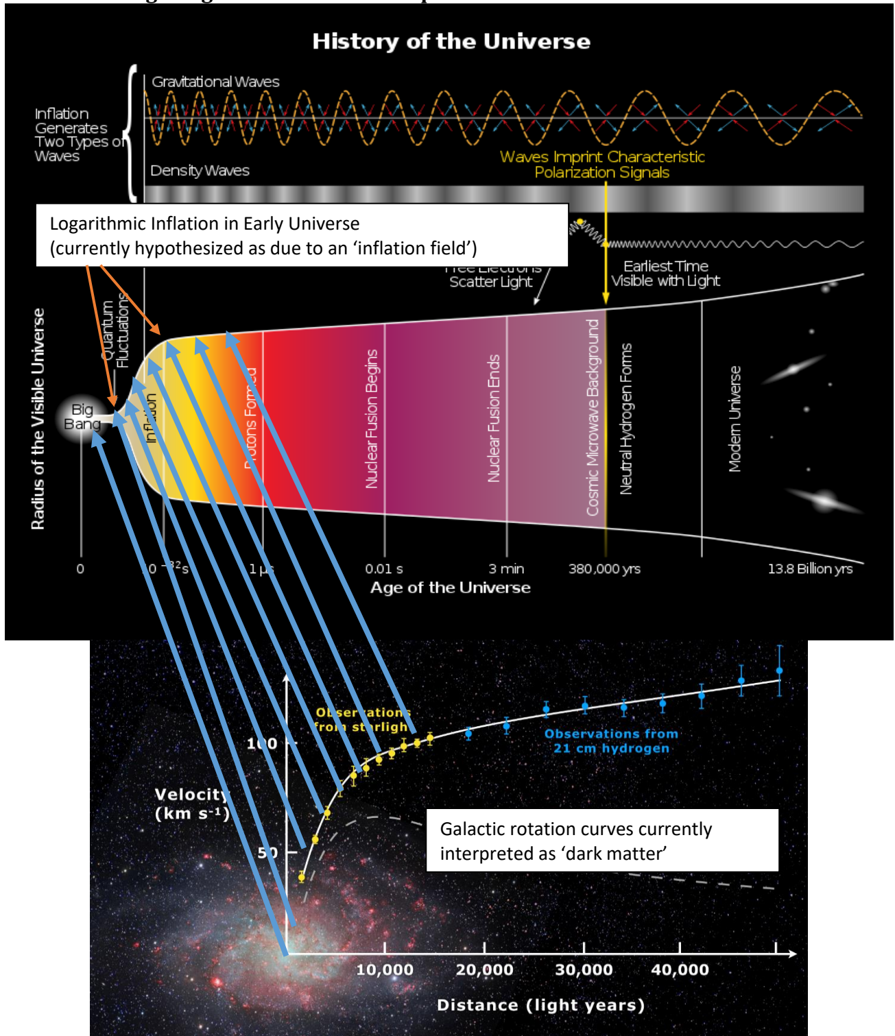
Figure 49. A Coincidence Too Big to Ignore? Big Bang-Inflation Curve Compared to Galactic Rotation Curves 28
