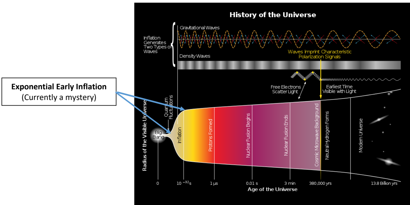
Figure 47. Exponential Early Acceleration of Universe’s Metric Expansion 26
