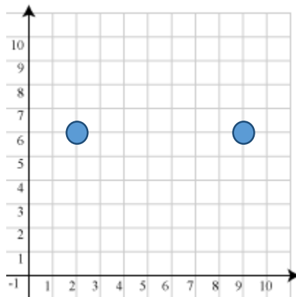
Two 'Particles' in Absolute Euclidean Space
