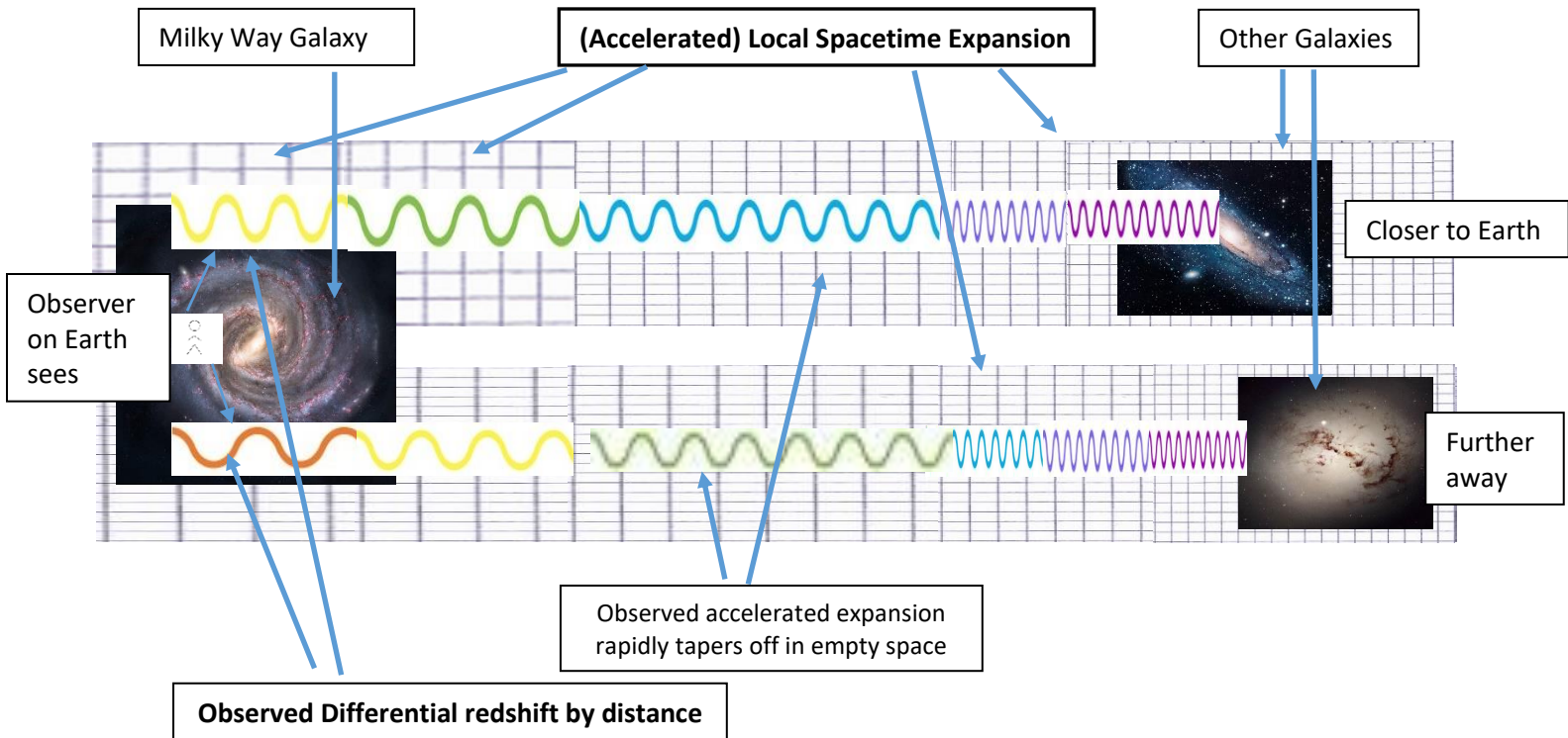
Figure 37. Redshift as Artifact of Mass-Energy Locally Accelerating Spacetime Metric Expansion 20
