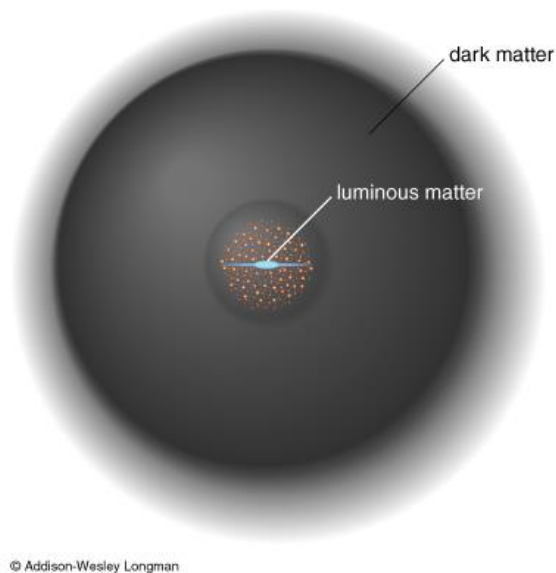
Figure 32. Hypothesized Galactic Dark Matter ‘Halos’ 16
