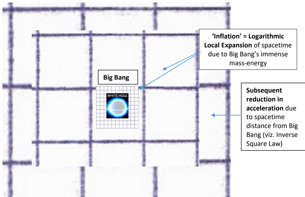
Figure 48. Early ‘Inflationary Epoch’ of the Universe as the Big Bang’s Gravity Exponentially Accelerating Local Spacetime Expansion 27
