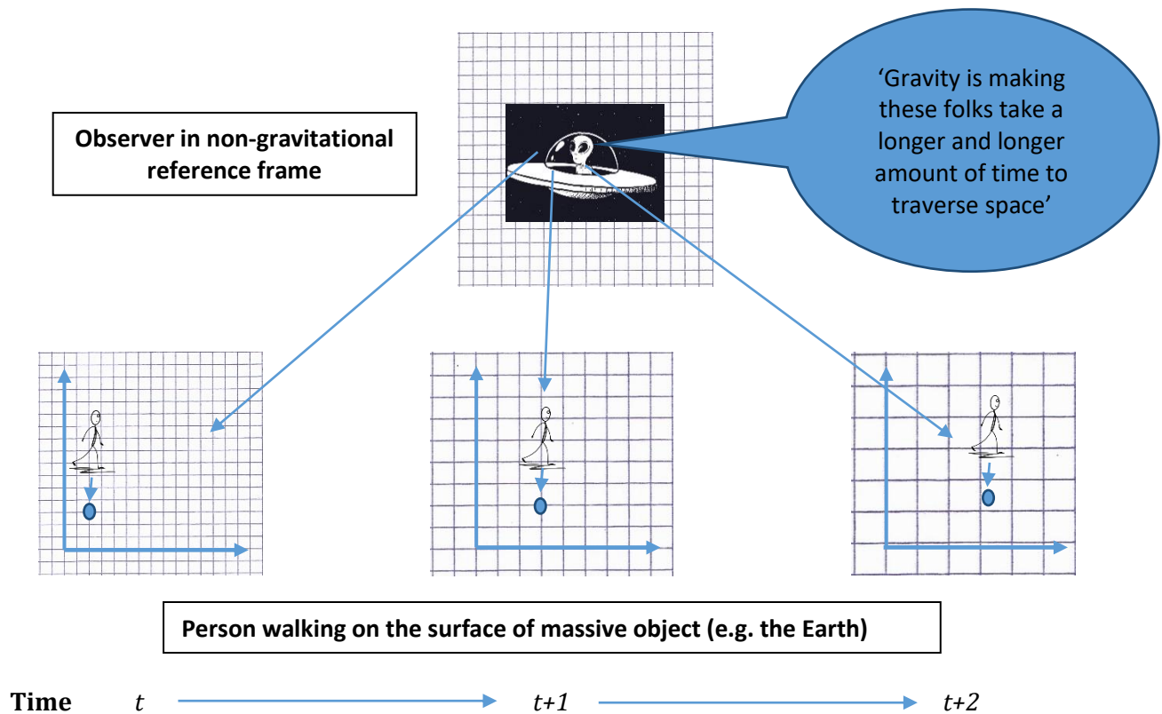
Figure 31. New Interpretation of Relativistic Spacetime Dilation 15
