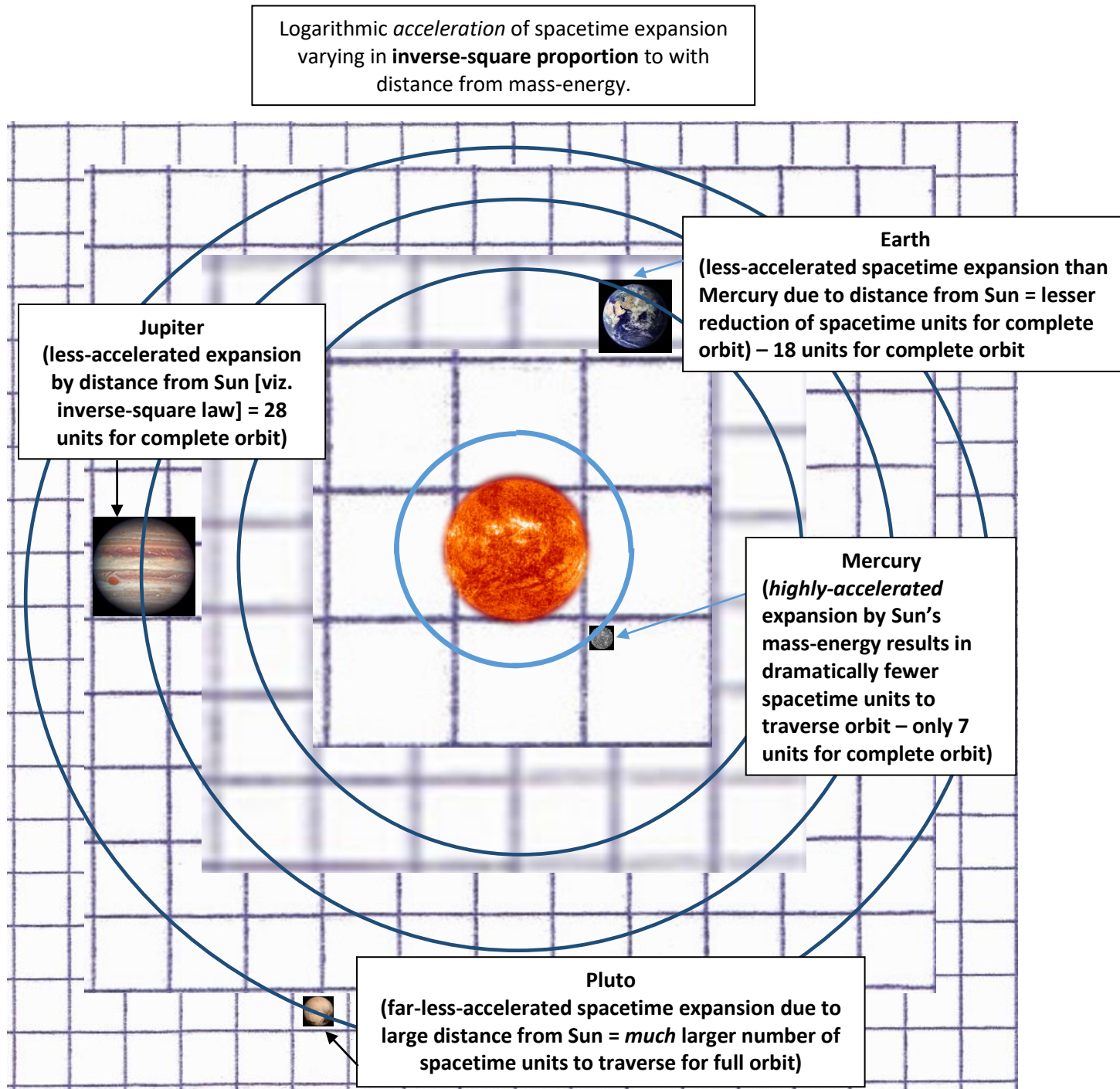
Figure 40. Re-Interpretation of Gravitational Motion (Illustrated in a Solar System) 22
