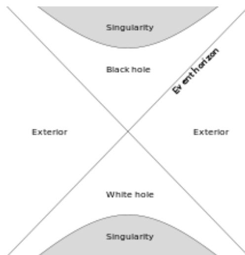
Figure 46. The Universe as ‘White Hole’ Generated by an Eternal Black Hole 25
