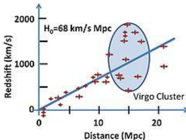
Figure 38. Deviations of Virgo Cluster Galaxies from Hubble’s Law 21
