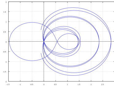
2 OUTPUT for \sigma = \frac{1}{2} as Gram points. Polar graph of \zeta(\frac{1}{2} + it) depicted as a two-dimensional figure (state) plotted along critical line for real values of t between -30 and +30 [viz, for s = \sigma \pm t range], horizontal axis: Re\{\zeta(\frac{1}{2} + it)\} , and vertical axis: Im\{\zeta(\frac{1}{2} + it)\} . Origin intercept points are present. There is manifestation of perfect Mirror symmetry about horizontal x-axis acting as the line of symmetry.
