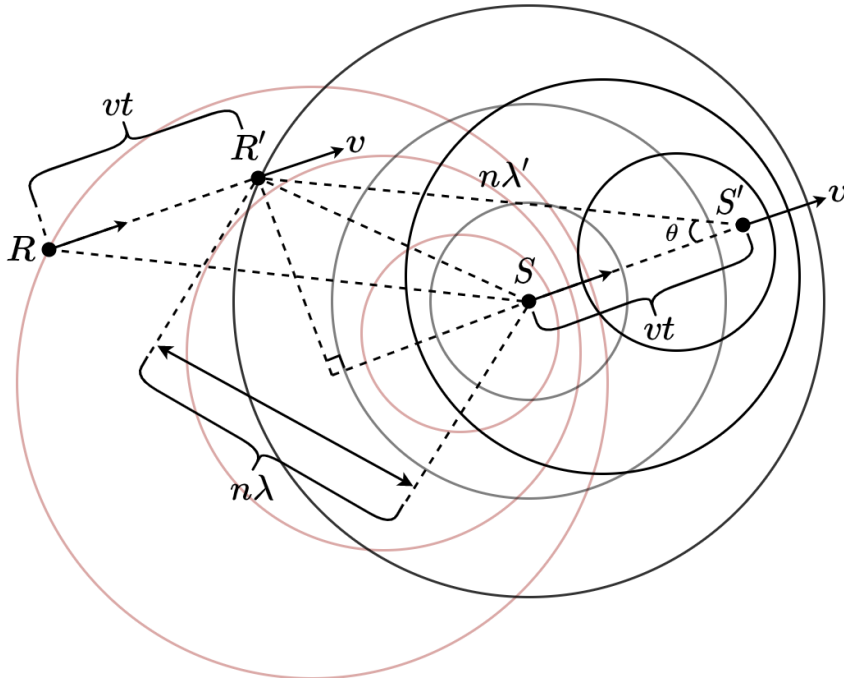
Figure 1: An emission source S and a receiver R moving at the same velocity in the same direction.
