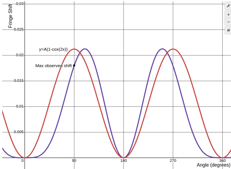
Figure 5: Predicted fringe shift displacements for \Delta_{FS}(\beta = 0.000784, \theta) (blue), with a cosine function (red) for comparison.
