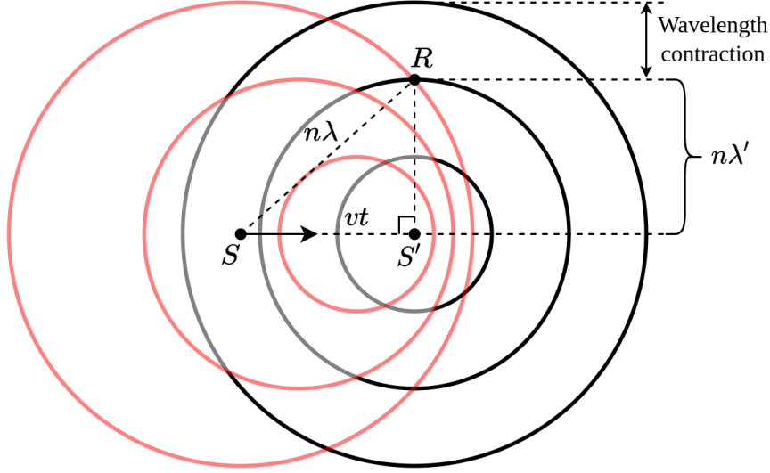
Figure 2: Transverse Doppler shift for a moving source.
