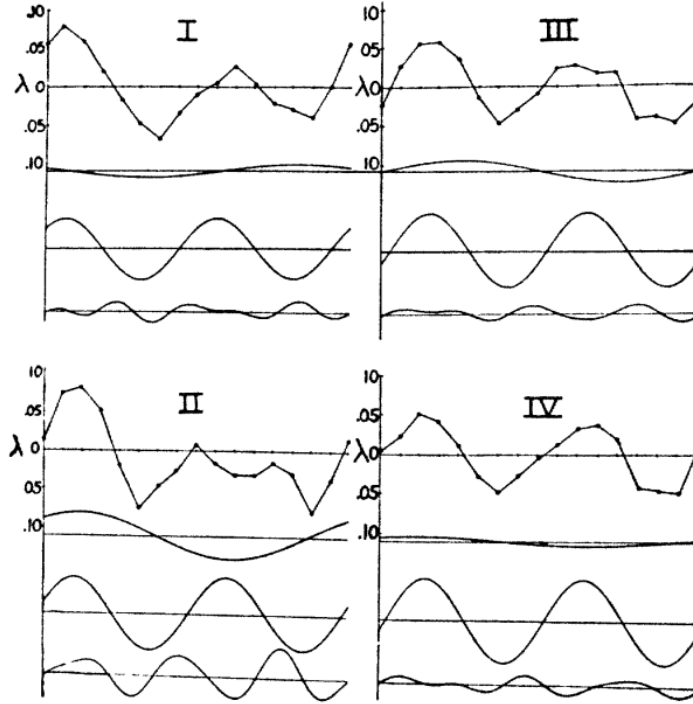
FIG. 21. Harmonic analysis of ether-drift observations.
