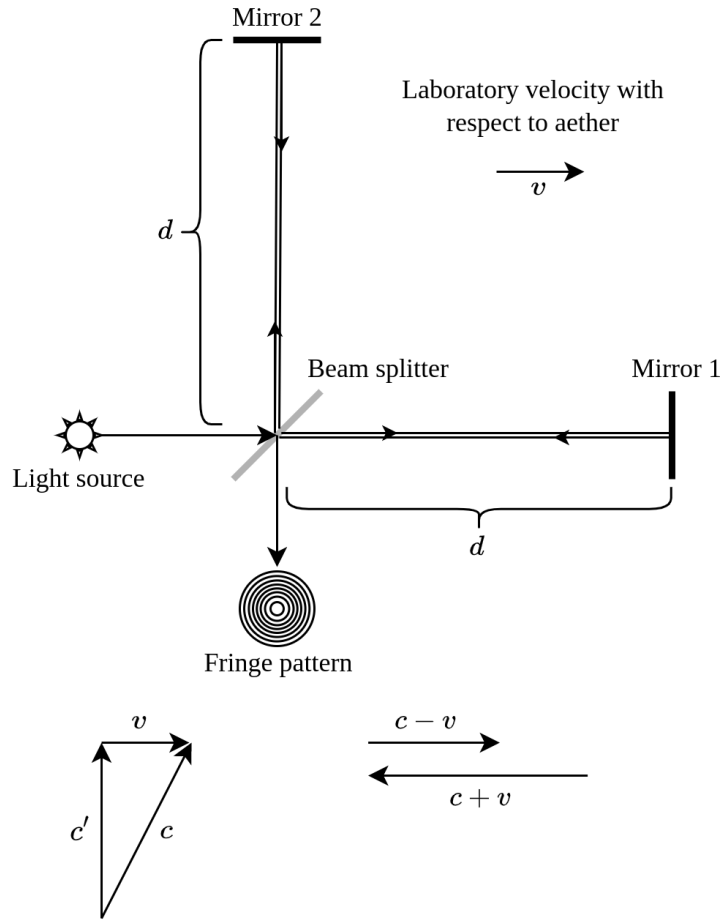
Figure 3: Experimental setup for the Michelson-Morley interferometer.
