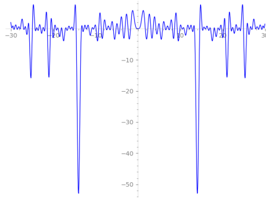
Figure 16. Graph of Z-function along [Analytically normalized] \Re(s) = \frac{1}{2} -critical line for -\infty < t < \infty depicting UNIQUE nontrivial zeros spectrum for Elliptic curve LMFDB label 234446.a1 [with non-zero Analytic rank of 4]. Note **Line Symmetry of vertical y-axis and trajectory intersecting Origin point. Integral points are (-10, 7), (-10, 3), (-9, 19), (-9, -10), (-8, 23), (-8, -15), (-7, 25), (-7, -18), (-4, 25), (-4, -21), (0, 17), (0, -17), (1, 14), (1, -15), (3, 7), (3, -10), (4, 3), (4, -7), (5, -2), (5, -3), (6, -1), (6, -5), (7, 3), (7, -10), (8, 7), (8, -15), (12, 25), (12, -37), (13, 30), (13, -43), (22, 83), (22, -105), (27, 118), (27, -145), (29, 133), (29, -162), (38, 207), (38, -245), (60, 427), (60, -487), (70, 543), (70, -613), (91, 815), (91, -906), (123, 1295), (123, -1418), (129, 1393), (129, -1522), (176, 2239), (176, -2415), (292, 4835), (292, -5127), (992, 30735), (992, -31727), (1140, 37907), (1140, -39047), (1656, 66545), (1656, -68201), (4532, 302803), (4532, -307335), (10583, 1083382), (10583, -1093965), (19405, 2693397), (19405, -2712802).
