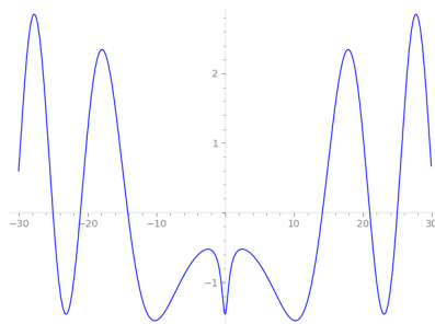
Figure 11. Graph of Z-function along \Re(s) = \frac{1}{2} -critical line for -\infty < t < \infty depicting UNIQUE nontrivial zeros spectrum for [Analytic rank 0] Dirichlet eta function \eta(s) ; the Analytic continuation of Riemann zeta function \zeta(s) . Note **Line Symmetry of vertical y-axis and trajectory DO NOT intersect Origin point. Integral basis 1. [An integral basis of a number field K is a \mathbb{Z} -basis for ring of integers of K . This is also a \mathbb{Q} -basis for K .]
