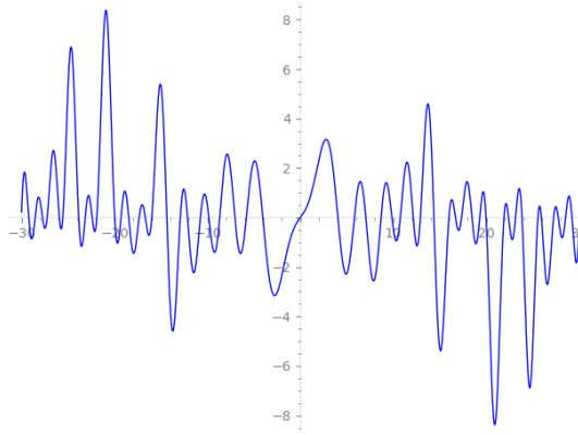
Figure 13. Graph of Z-function along [Analytically normalized] \Re(s) = \frac{1}{2} -critical line for -\infty < t < \infty depicting UNIQUE nontrivial zeros spectrum for Elliptic curve LMFDB label 65.a1 [with non-zero Analytic rank of 1]. Note **Point Symmetry of Origin point and trajectory intersecting Origin point. Integral points are (-1, 1) , (-1, 0) , (0, 0) , (1, 0) , (1, -1) , (4, 6) , (4, -10) .
