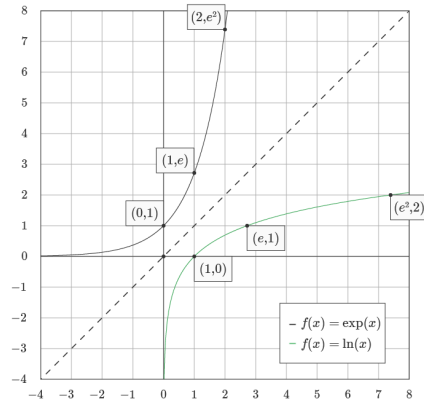
Figure 8. Natural logarithm function \log_e x or \ln(x) . Natural exponential function \exp(x) or e^x . The graphs of \log_e x and its inverse e^x are symmetric w.r.t. line y = x . Geometrically, this denote diagonal symmetry of the two functions; viz, \ln(e^x) = x and e^{\ln(x)} = x .
