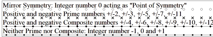
Integer number line (from -12 to +12 depicted on the horizontal or x-axis) -12 -11 -10 -9 -8 -7 -6 -5 -4 -3 -2 -1 0 1 2 3 4 5 6 7 8 9 10 11 12
