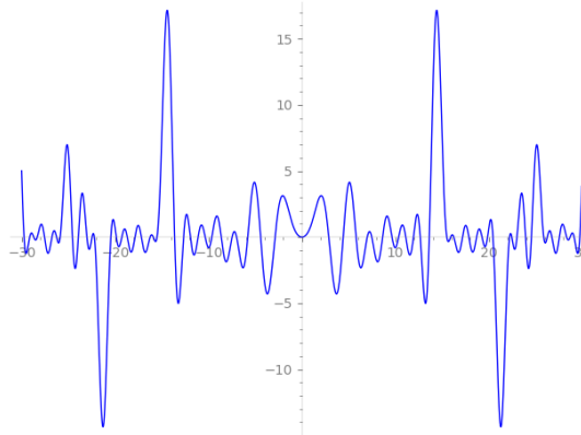
Figure 14. Graph of Z-function along [Analytically normalized] \Re(s) = \frac{1}{2} -critical line for -\infty < t < \infty depicting UNIQUE nontrivial zeros spectrum for Elliptic curve LMFDB label 389.a1 [with non-zero Analytic rank of 2]. Note **Line Symmetry of vertical y-axis and trajectory intersecting Origin point. Integral points are (-2, 0) , (-2, -1) , (-1, 1) , (-1, -2) , (0, 0) , (0, -1) , (1, 0) , (1, -1) , (3, 5) , (3, -6) , (4, 8) , (4, -9) , (6, 15) , (6, -16) , (39, 246) , (39, -247) , (133, 1539) , (133, -1540) , (188, 2584) , (188, -2585) .
