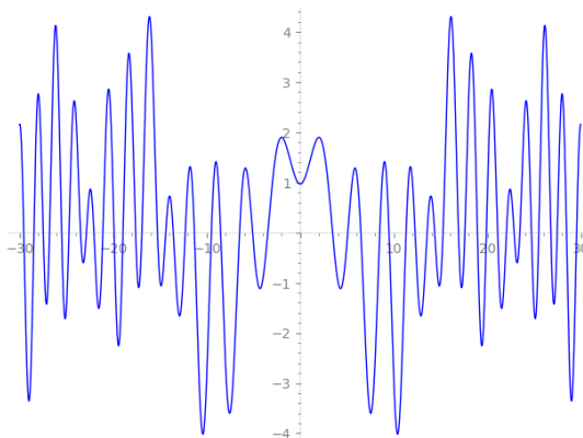
Figure 12. Graph of Z-function along [Analytically normalized] \Re(s) = \frac{1}{2} -critical line for -\infty < t < \infty depicting UNIQUE nontrivial zeros spectrum for Elliptic curve LMFDB label 49.a4 [with Analytic rank of 0]. Note **Line Symmetry of vertical y-axis and trajectory DO NOT intersecting Origin point. Integral point is (2, -1).
