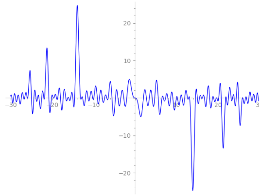
Figure 15. Graph of Z-function along [Analytically normalized] \Re(s) = \frac{1}{2} -critical line for -\infty < t < \infty depicting UNIQUE nontrivial zeros spectrum for Elliptic curve LMFDB label 21858.a1 [with non-zero Analytic rank of 3]. Note **Point Symmetry of Origin point and trajectory intersecting Origin point. Integral points are (-7, 5), (-7, 2), (-6, 12), (-6, -6), (-4, 14), (-4, -10), (-2, 12), (-2, -10), (1, 5), (1, -6), (2, 2), (2, -4), (3, 0), (3, -3), (4, 2), (4, -6), (5, 5), (5, -10), (7, 12), (7, -19), (11, 29), (11, -40), (14, 44), (14, -58), (22, 92), (22, -114), (30, 150), (30, -180), (68, 530), (68, -598), (119, 1244), (119, -1363), (122, 1292), (122, -1414), (137, 1541), (137, -1678), (786, 21660), (786, -22446), (1069, 34437), (1069, -35506), (38746, 7607514), (38746, -7646260), (783868, 693616502), (783868, -694400370) .
