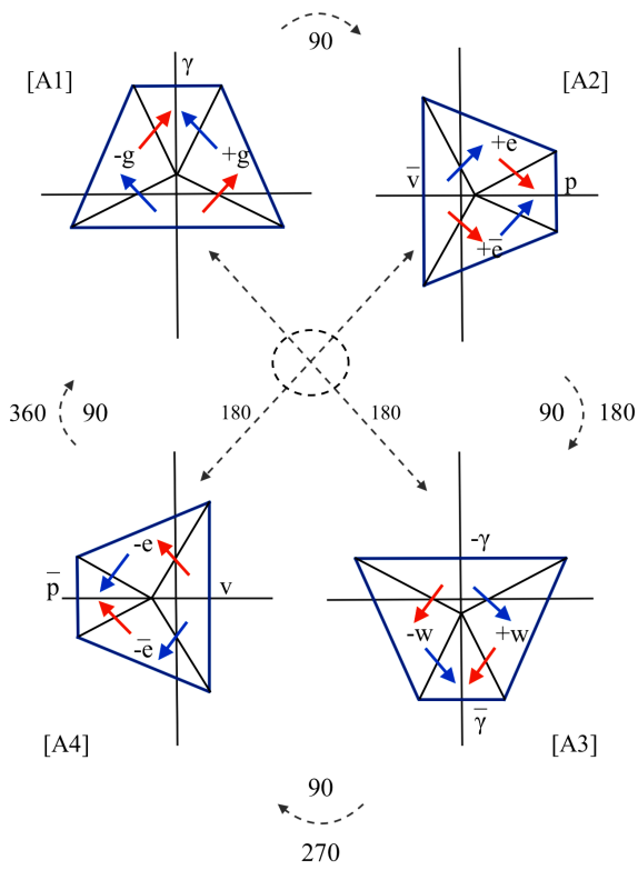
Figure 3: Illustration of the rotational system
