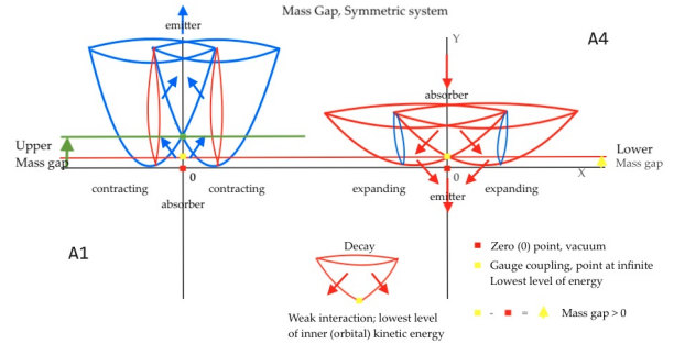
Figure 8: Mass gap in the symmetric system
