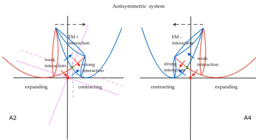
Figure 7: Mass gap in the antisymmetric system
