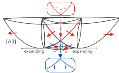
Figure 9: symmetric system: Singularities in central subfields represented as abrupt changes of curvature.
