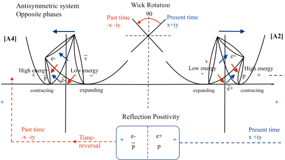
Figure 5: Depiction of reflection positivity in the antisymmetric system
