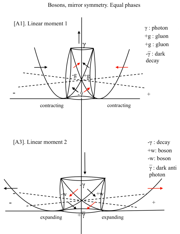
Figure 4: Polarization in the symmetric system: The central subfield moves up or down along the vertical axis as the transverse subfields expand or contract
