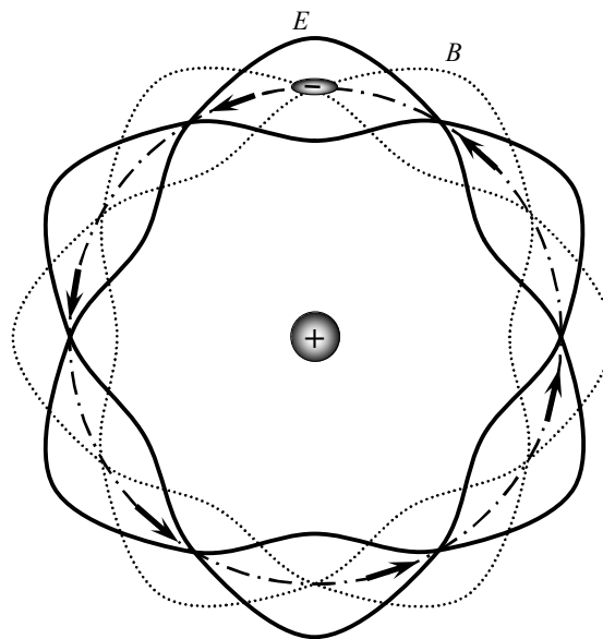
Fig. 6. Spin of electromagnetic field standing wave and electron spin
