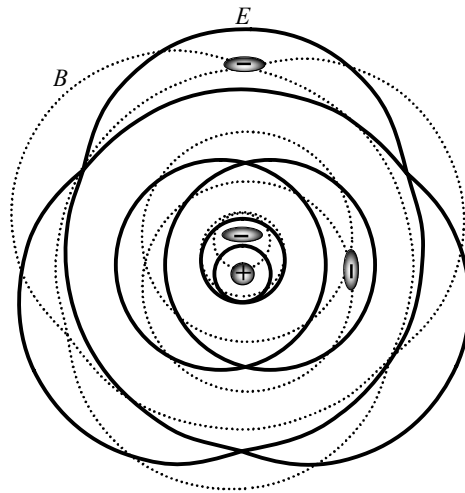
Fig. 5. The shape of the generalized field fluctuation of hydrogen-like atoms
