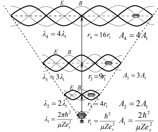
Fig. 4. Development diagram of the electromagnetic field standing wave of a hydrogen-like atom at four energy levels.
