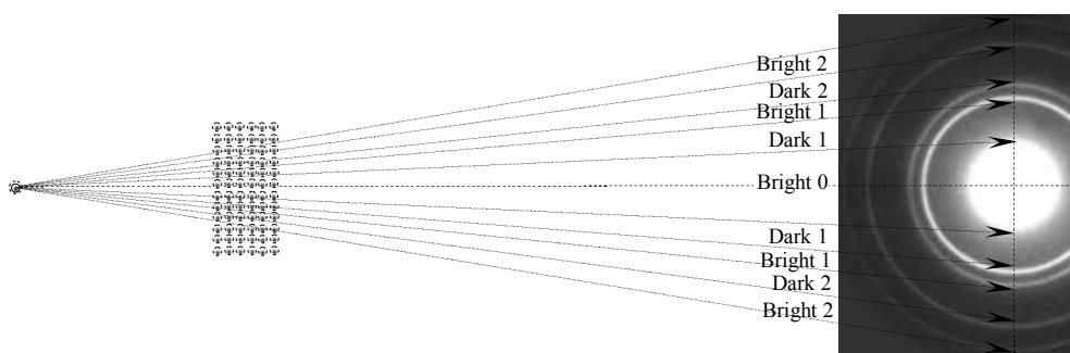
Fig. 16. Examples of Davisson-Gemmer Experimental Analysis Patterns 2
