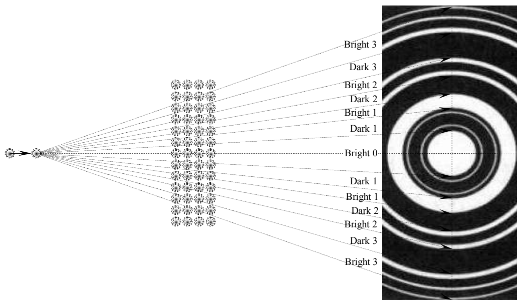
Fig. 15. Examples of Davisson-Gemmer Experimental Analysis Patterns 1
