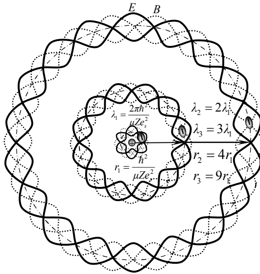
Fig. 3. Electromagnetic field standing waves of hydrogen-like atoms at three energy levels.
