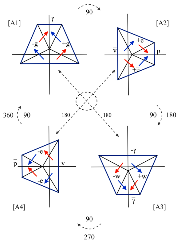
Figure 9: Reflection positivity in the antisymmetric system
