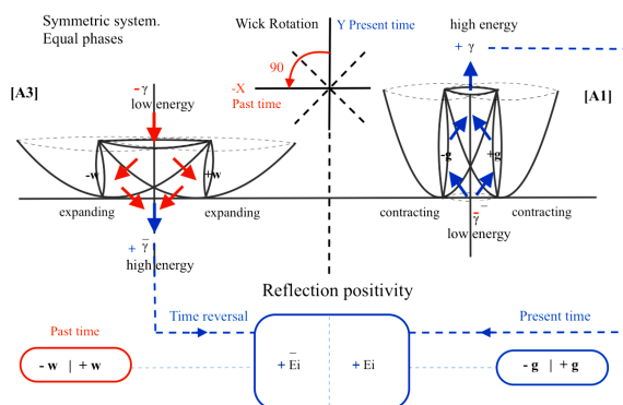
Figure 10: Reflection positivity in the Symmetric system
