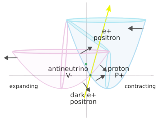
Figure 4: subatomic particles in the fermionic antisymmetric system when the right field contracts and the left expands.
