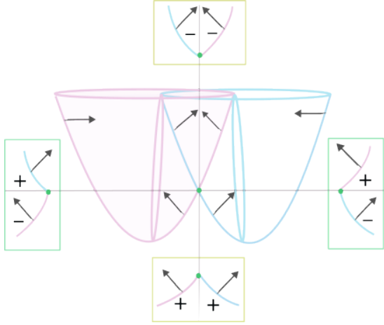
Figure 2: Singularities, as abrupt changes in curvature, inside the nuclear subfields in the bosonic system when both intersecting fields contract.
