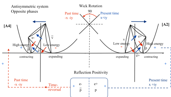
Figure 9: Reflection positivity in the antisymmetric system
