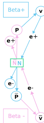
Figure 5: Diagram that illustrates the neutron as an intermediate state during proton-antiproton transformations in beta decay reactions, showing the paths followed and the particles involved in each case.
