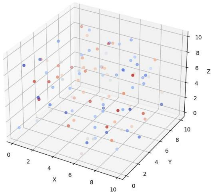
Figure 1: 3D Scatter Plot of Grain Distribution and Charges in the Spacetime Matrix.
