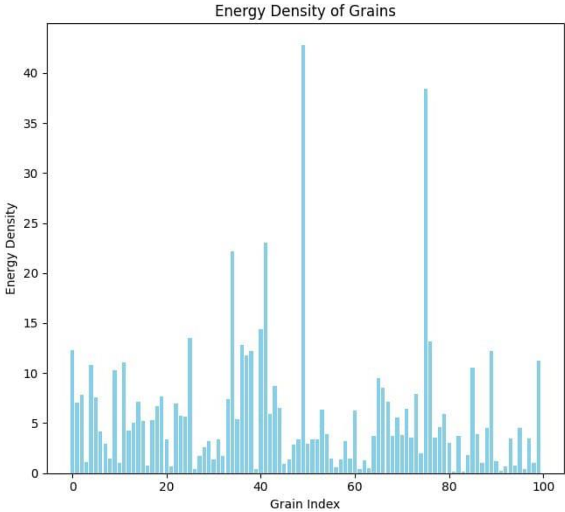
Figure 2: Energy Density of Grains in the Spacetime Matrix.
