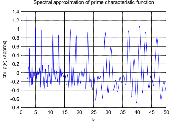
Figure 2: Spectral approximation of prime characteristic function. The horizontal axis k ranges from 0 to 50. The vertical axis is labeled " \chi_p(k) (approx)".
