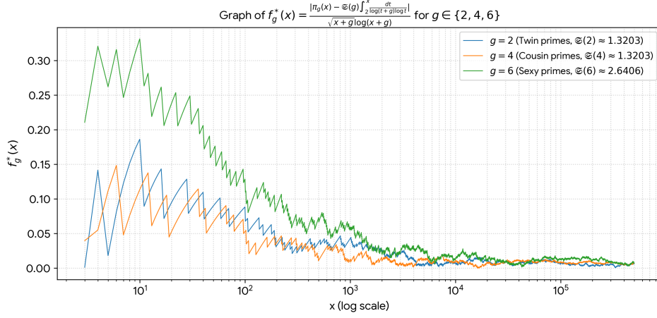
Figure 7: Relative error of the asymptotic estimate of the prime pair function \pi_g(x) for given gaps g
