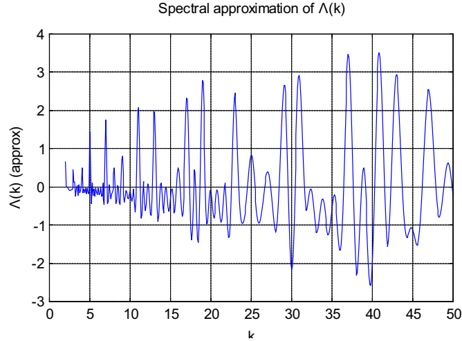
Figure 1: Spectral approximation of \Lambda(k) showing the approximate values of the von Mangoldt function against k on the horizontal axis. The horizontal axis ranges from 0 to 50.
