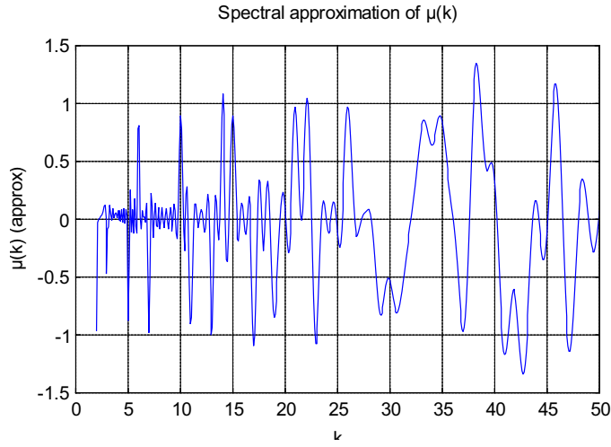
Figure 3: Spectral approximation of \mu(k) showing the approximate values of the Möbius function plotted against k , which ranges from 0 to 50 on the horizontal axis.
