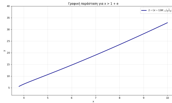
Figure 5: Inverse prime counting function \pi^{-1}(x) approximation graph.
