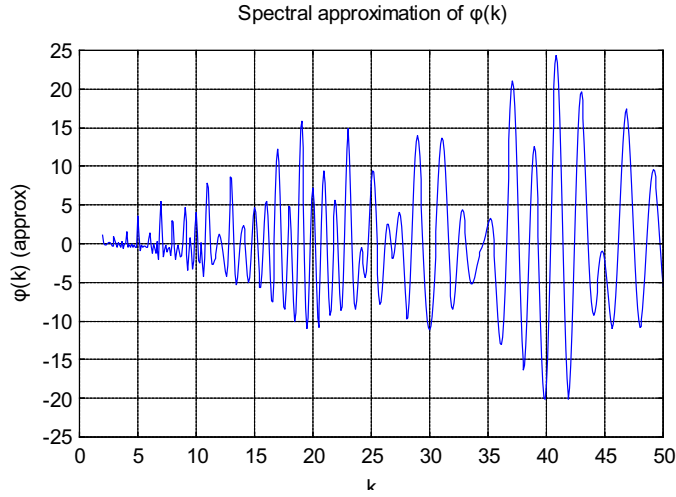
Figure 4: Spectral approximation of \phi(k) showing the approximate values of the Euler totient function, plotted against k values on the horizontal axis from 0 to 50.
